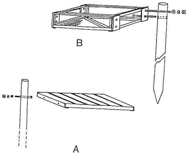
Fig. 2. Platform structures. A. This basic version consists of four heavy pipe legs that bolt to a simple angle-iron frame (36 x 48 inches) supporting the wooden platform. Resistance to ice damage can be increased somewhat by constructing a rock crib between the legs. B. The reinforced platform increases ice resistance substantially because structural rigidity of the sturdy 36- x 42-inch frame is transferred to the legs. Two bales are wired to the simple platform or wedged into the upper framework of the reinforced platform.
